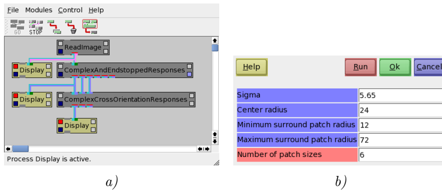
Figure 4. a) TiViPE network. b) Parameters used for cross orientation type of cells.
