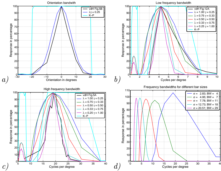
Figure 2: Measured and modeled response profiles of grating cells. a) Orientation, b) low frequency, and c) high frequency profiles. d) Frequency profiles for different preferred bar width sizes (BW = 4, 7, 11, 18, and 29 pixels). Cycles per degree have arbitrary units. Parameters used for d) are \lambda = 1 and \gamma = 0.25 .
