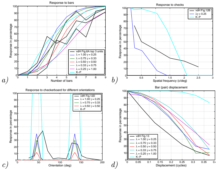
Figure 3: Measured and modeled properties of grating cells. a) Response profile for increasing number of bars. b) Response to checks. c) Sensitivity to different orientations of a checkerboard pattern. d) Responses to increasing shift of a pair of bars, the so-called Stresemann pattern.
