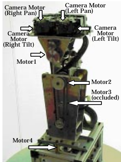
b) Mechanical structure
