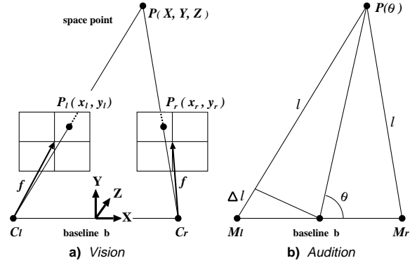
Figure 3: Epipolar geometry for localization
